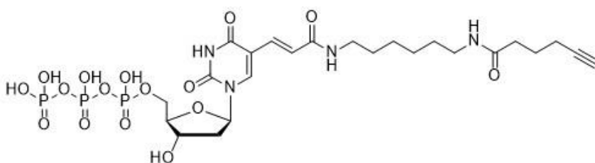
Structure 15-Alkyne-dUTP
